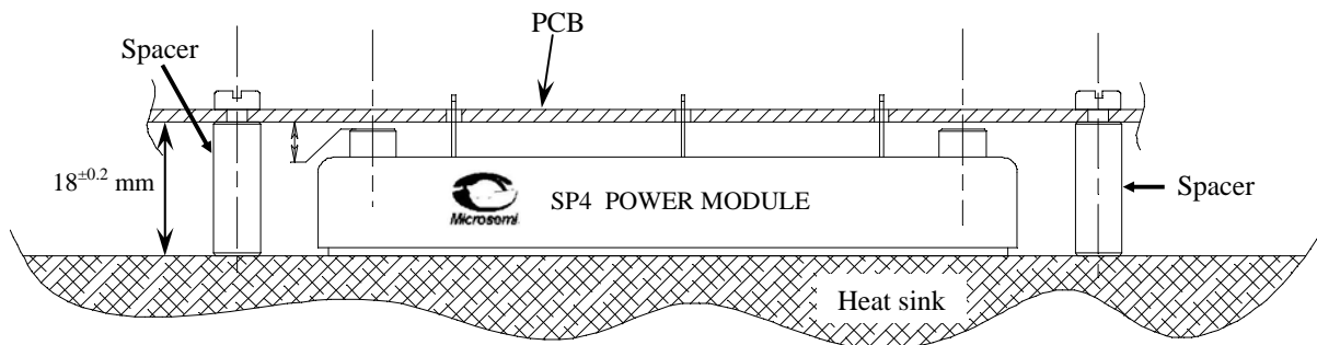
Fig 8: PCB screwed onto the metallic spacers.
