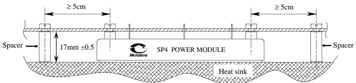
fig 7: Spacers used on large PCB.
