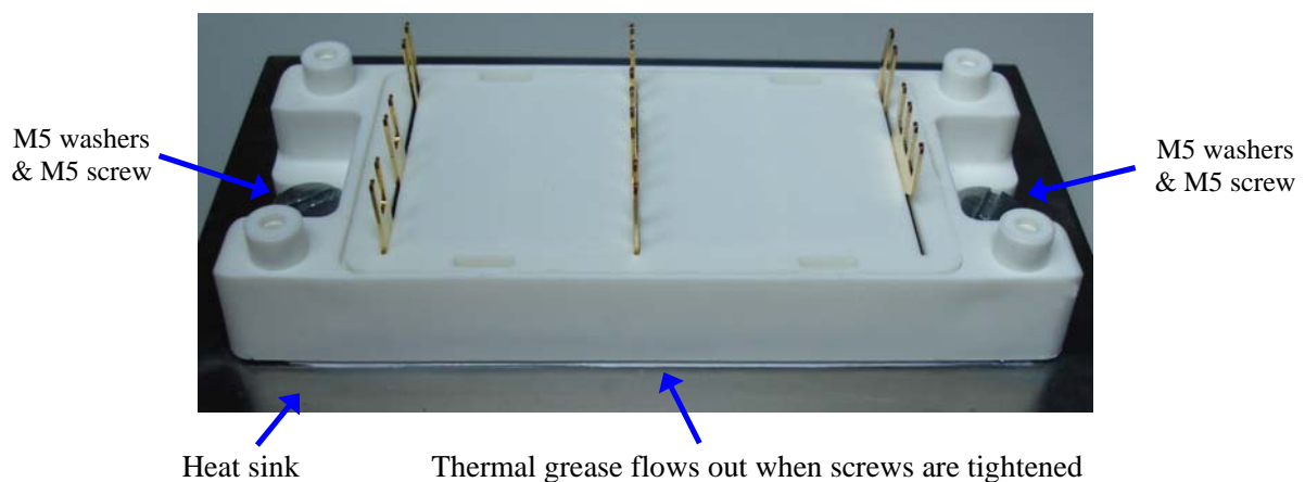
fig 3: Proper application of thermal grease to the power module.
