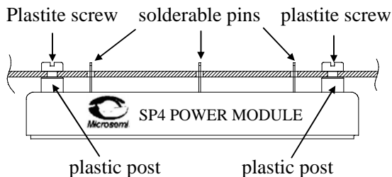
fig 1: PCB mounted on SP4 power module.
