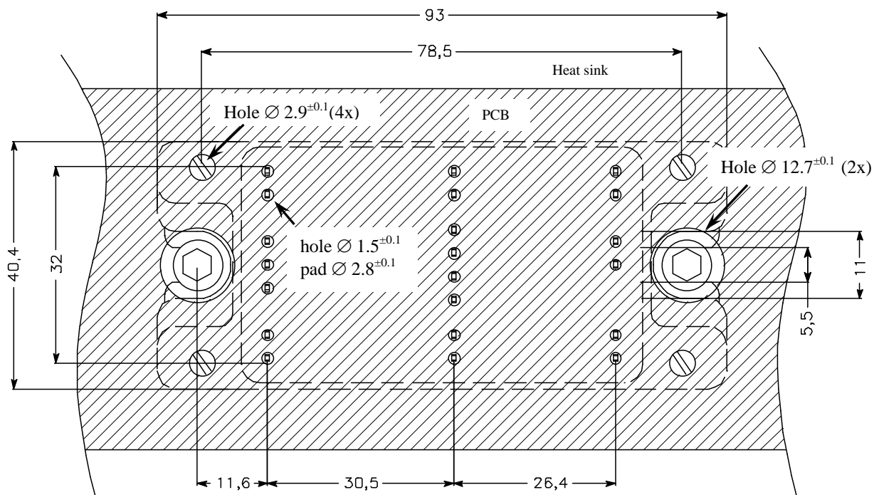
Fig 5: pad and hole diameters (in millimeters).
