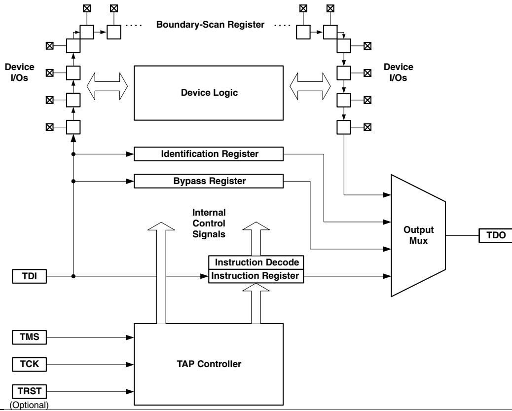
Figure 4 • JTAG Boundary-Scan Test Circuitry
